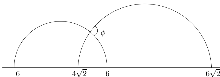
Figure 5.6.3: The internal angle between two circles
