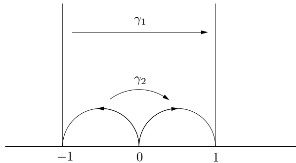
Figure 29.2.2: A fundamental domain for the free group on 2 generators
