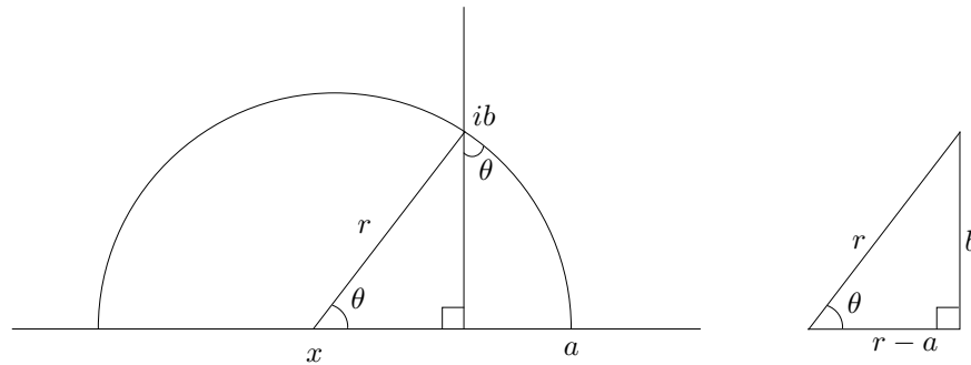
Figure 30.3: The (Euclidean) triangle with vertices at x, 0, ib
