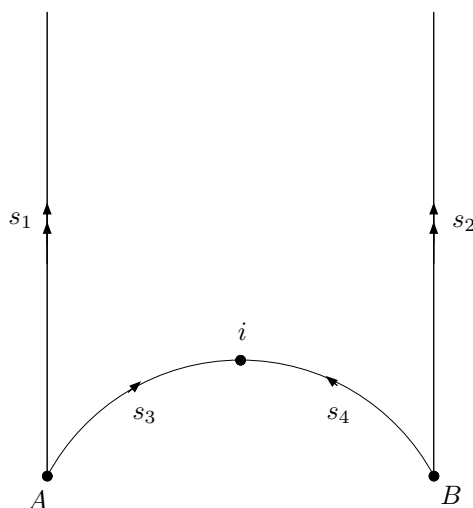
Figure 30.11: A fundamental domain and side-pairing transformations for the modular group
