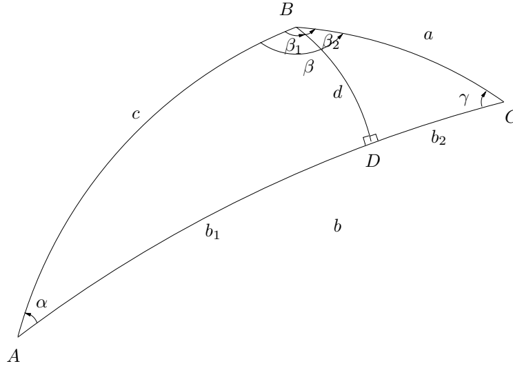
Figure 30.5: The sine rule
