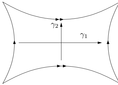
Figure 29.2.1: A hyperbolic quadrilateral with opposite sides paired
