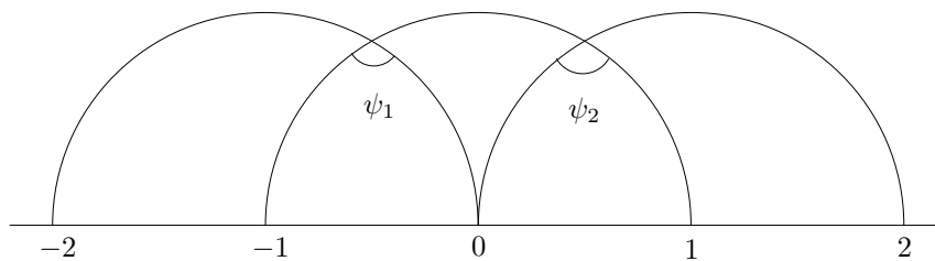
Figure 30.4: The angles \psi_1, \psi_2
