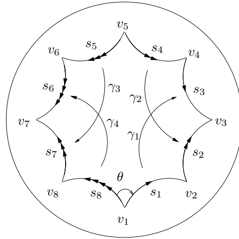
Figure 30.10: See the solution to Exercise 21.2
