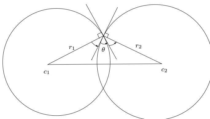
Figure 30.1: The Euclidean triangle with vertices at c_1, c_2 and the point of intersection
