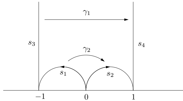
Figure 30.8: A fundamental domain for the free group on 2 generators
