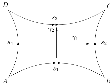
Figure 30.7: A hyperbolic quadrilateral
