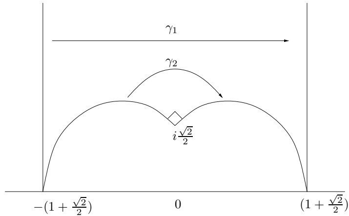
Figure 29.2.3: A hyperbolic quadrilateral
