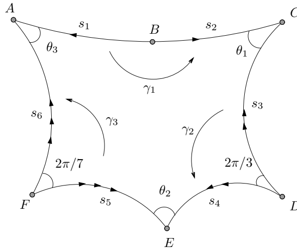
Figure 30.9: Labelling the hyperbolic polygon, remembering to add an extra vertex to the side that is paired with itself
