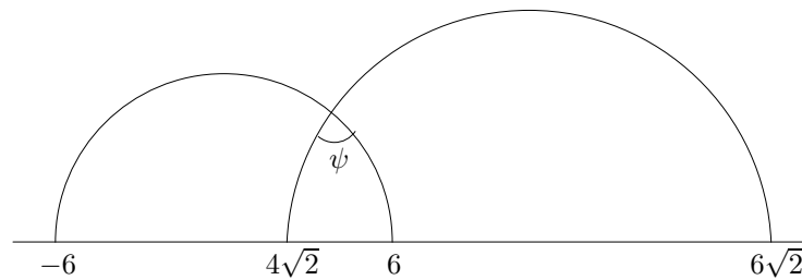
Figure 30.2: The angle \psi
