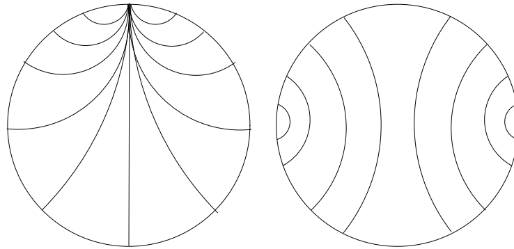
Figure 30.6: Solution to Exercise ex:examplesoftwotessellations
