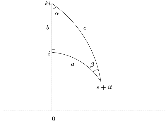
Figure 5.7.6: Without loss of generality, we can assume that \Delta has vertices at i, ki and s + it
