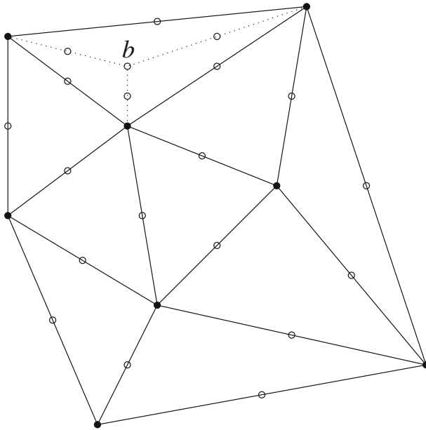
Fig. 5 An illustration of Case 2
