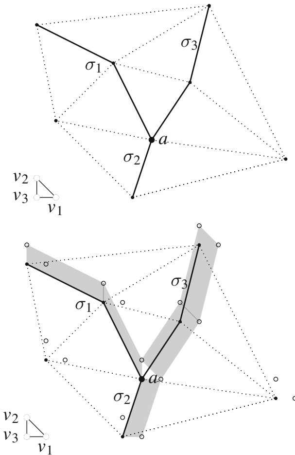
Fig. 6 A proper star with respect to v_1, v_2, v_3 centered at a . On the right, parallelgrams based on the proper star
