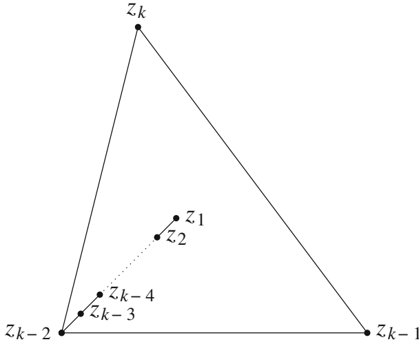
Fig. 1 An illustration of case (b) in Theorem 1.2
