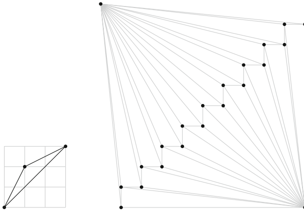
Fig. 2 An illustration of the example described in Proposition 1.6
