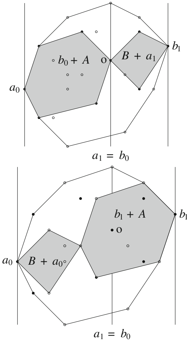
Fig. 7 An illustration of the proof of Claim 1
