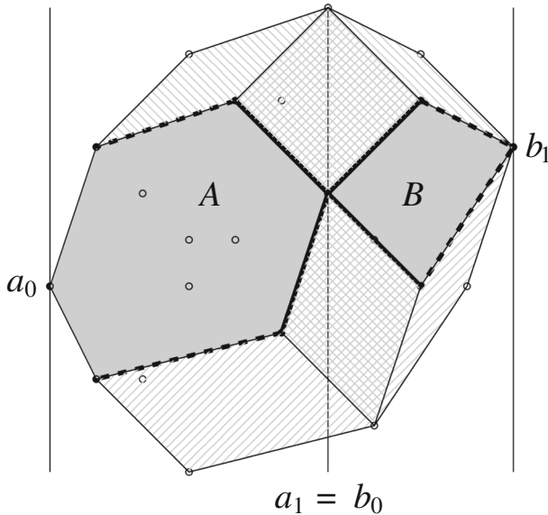
Fig. 8 An illustration of the parallelograms of the mixed subdivision in Case 1
