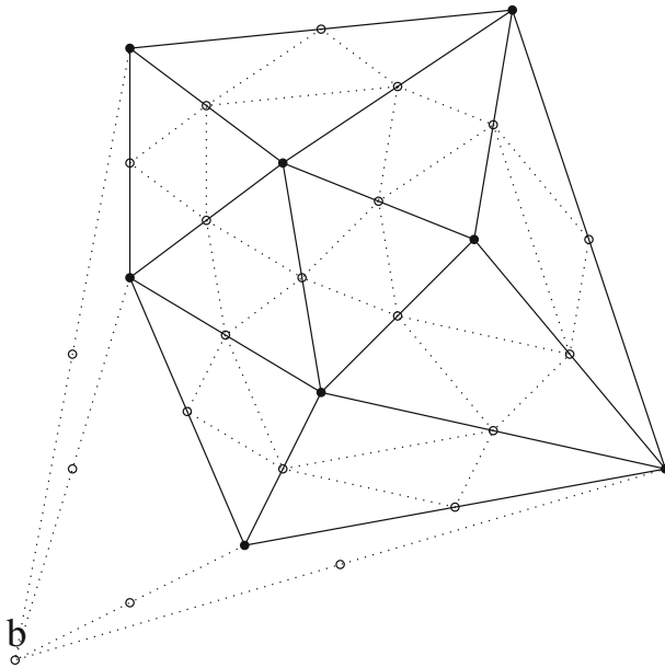
Fig. 4 An illustration of Case 1
