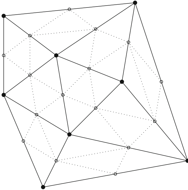
Fig. 3 A triangulation and its midpoints
