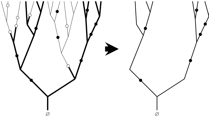
FIG. 1. Scaling of the marked binary branching tree. On the left: At time t , points in \Pi_t are still closed and marked with white circles, while points in \Pi_0 \setminus \Pi_t have already opened and are marked with black circles. On the right: Removing the loose ends from the open cluster at the root yields a stretched version of the original marked binary branching tree.
