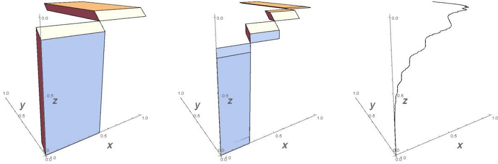
FIGURE 4. Linearly parametrized de Rham curve with parameter \omega = 1/10 . Left: The image of the unit cube w.r.t the IFS generating the graph of the de Rham curve. Middle: The second iteration. Right: The curve itself.
