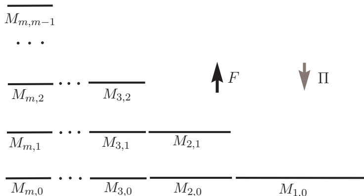
FIGURE 2. The structure of cells M_{m,i} in the space M . The “bottom level” of M is the induced phase space \mathcal{M} = \bigcup_{m=0}^{\infty} \mathcal{M}_m = \bigcup_{m=0}^{\infty} M_{m,0} . The map F moves each cell one level up, but the top cell in each column is mapped back down to \mathcal{M} . The projection \Pi (Section 6) collapses each column \bigcup_{i=0}^{m-1} M_{m,i} onto its bottom element M_{m,0} = \mathcal{M}_m .
