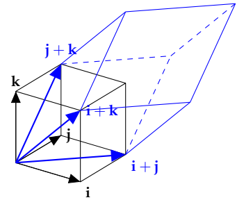
1.31. ábra: (\mathbf{i} + \mathbf{j})(\mathbf{j} + \mathbf{k})(\mathbf{k} + \mathbf{i}) = 2
